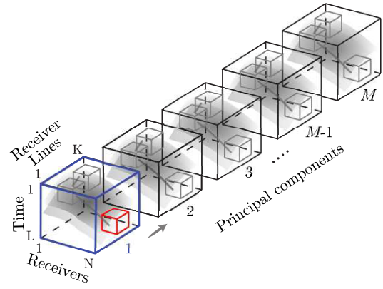
Fig. 2. Illustration of multichannel BM4D cube-matching for different PCs of \mathbf{v}_k , showing the matching of three cubes. The cube-matching is performed only on the first PC; the resulting cube positions are then repeated across every component 1, ..., M to form the corresponding groups of cubes.
