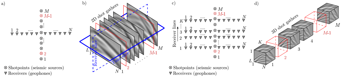
Fig. 1. (a) Cross-spread [4], [9] and (c) swath geometry [12]. (b) and (d) Three-dimensional and 4-D tensor presentation for the subsampled acquisitions from (a) and (c), respectively, by removing the shotpoints at 2 and M - 1 .
