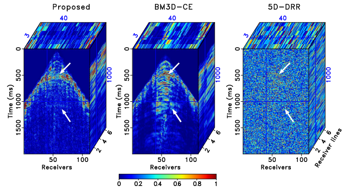
Fig. 3. Three-dimensional absolute differences between the original shot gather 4 and those interpolated by the proposed, BM3D-CE, and 5D-DRR methods. Note that the slices are at 1000 ms, receiver 40, and receiver line 3, respectively.
