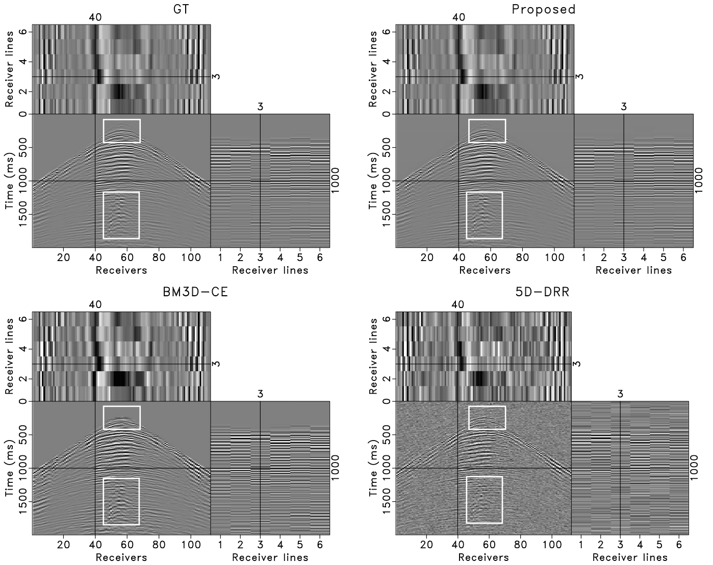
Fig. 4. Comparison of the interpolated 3-D shot gather 4 using the slices at time 1000 ms, receiver 40, and receiver line 3. The white box highlights the ground roll accurately reconstructed by the proposed method. The upper box shows the first arrivals omitted by the BM3D-CE method.
